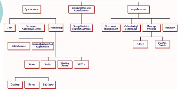
CSCW Software Family Tree
