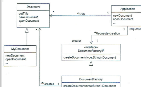
FIGURE 5.2 Application framework with document factory.
