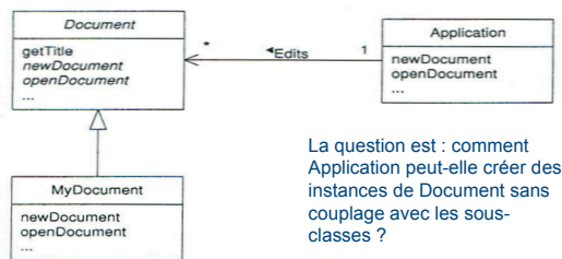
FIGURE 5.1 Application framework.
