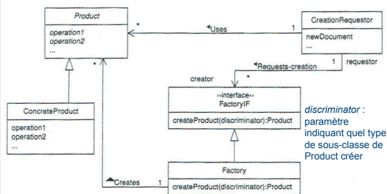
FIGURE 5.3 Factory method pattern.
