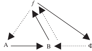
Fig. 6. This diagram represents Rosen's explanation of the closure of an (M, R) system. The broken arrows indicate that a function (located at the start of the arrow) uses a variable (at the destination) to produce a result. Each solid arrow indicates a transformation. The interesting aspect of this diagram is that every biological function (metabolism f ), replacement (\Phi) or organizational invariance (the implied \beta which is equivalent to some element b \in B ) is entailed by another element in the diagram. No outside causality is needed. This is the basic bootstrapping property of a living system that justifies Rosen's statement that "Organisms are closed to efficient causes". A full discussion is in Chapter 10 of Life Itself , but note that Diagram 10.5C therein contains an error in defining the arrows.
