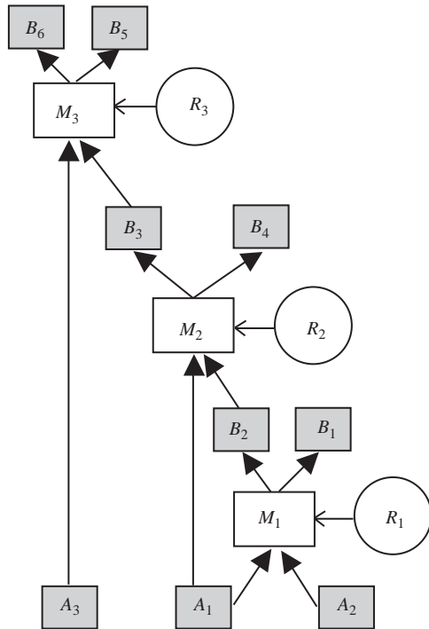
Fig. 3. A small (M, R) system with three enzymes (“components”) ( M_1, M_2, M_3 ) and three “repairers” ( R_1, R_2, R_3 ). Associated with each M_i is a subsystem (a collection of processes) R_i that maintains by replacement a functional amount of each M_i . Each subsystem is specific to a particular enzyme. Rosen called this process repair , but the term replacement indicates more clearly what is involved. For simplicity, we treat enzyme degradation as an uncatalysed and unavoidable process, though in real organisms much of it is catalysed.
