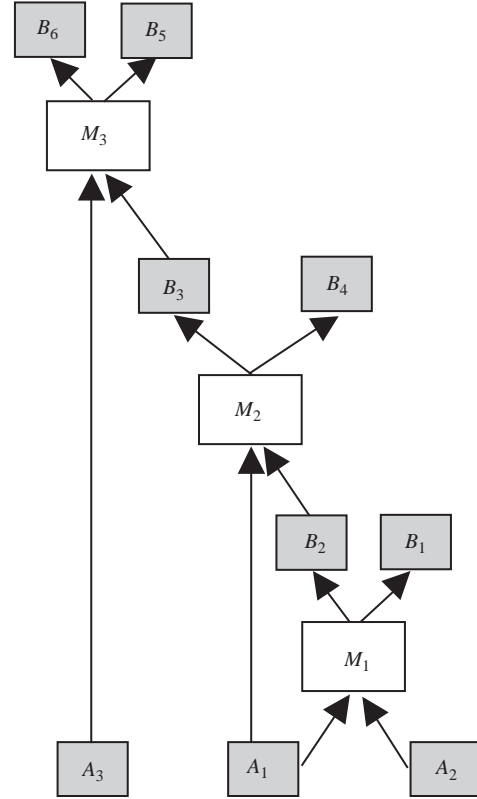
Fig. 1. An initial view of a metabolic network as a collection of catalysts ( components in Rosen’s terminology: see Table 1) ( M_1, M_2, M_3 ) that transform metabolites from specific sets ( A_1, A_2, A_3, \dots ) into specific sets ( B_1, B_2, B_3, \dots ).
