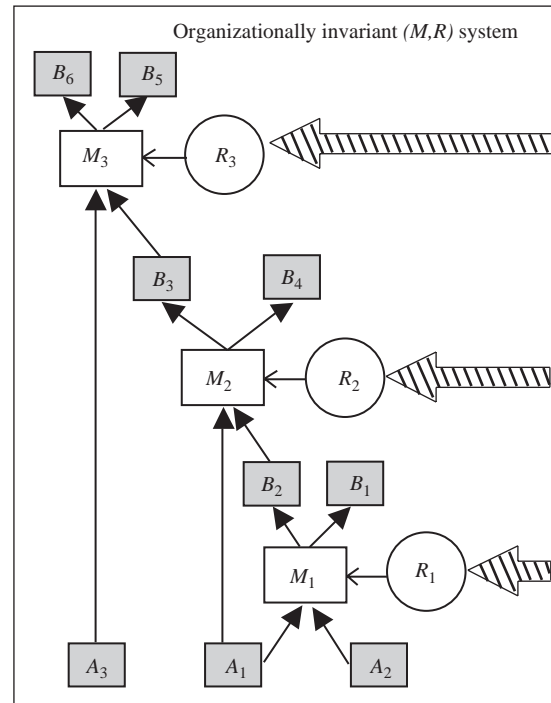
Fig. 4. Logical structure of an organizationally invariant (M, R) system (“replicative (M, R) system”). In this system the replacement of each R_i is a systemic property that depends on the system considered as a whole. The hatched arrows arriving at each R_i , and departing from the system’s border, represent this dependence. The proof that this dependence is possible constitutes Rosen’s central result.
