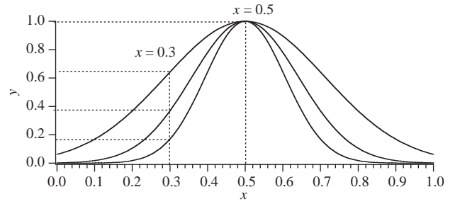
Fig. 5. Rigidity implied by invertible evaluations. Let X = Y = [0, 1] and H(X, Y) to be the infinite family of bell-shaped graphs ( y = f_x(x) = \exp(-((x - 0.5)/\alpha)^2) ) sketched in the figure. Note that Ev_x is one-to-one for almost every x in [0, 1] (for example at x = 0.3 ). The only exception is x = 0.5 because all curves collapse at this point.
