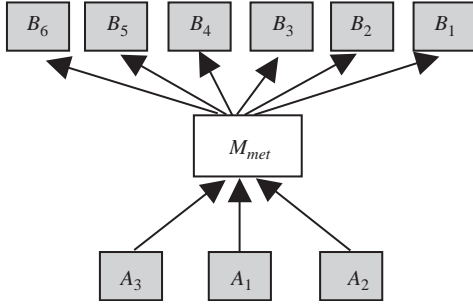
Fig. 2. The network of Fig. 1 viewed as the action of a single catalyst ( M_{met} ). All the intermediate steps have disappeared, though the intermediate metabolites ( B_2 and B_3 ) have not.
